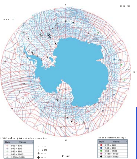
Fig. 4: Streamlines before SRM (1 SU = 100 m²/s) (blue), isobars [hPa] (red), SSM/I drift vectors [m/s] (blue), and cyclone positions calculated from ECMWF and SSM/I data (see legend).
