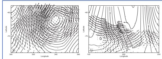
Fig. 1: Streamfunction by RM in 100 m²/s. Strong meridional streamline orientation corresponds well with drift vectors for Weddell sea area (left), but insufficiently for Ross sea area (right).
