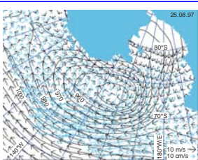
Fig. 1: Daily means of ECMWF wind vectors and isobars (black), and SSM/I sea ice drift vectors (blue). Positions of the displayed cyclone differ by about 10° longitude.
