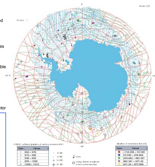
Fig. 5: SRM streamlines (1 SU = 100 m²/s) (green), isobars [hPa] (red), SSM/I drift vectors [m/s] (blue), and cyclone positions calculated from ECMWF- and SRM SSM/I data (see legend).
