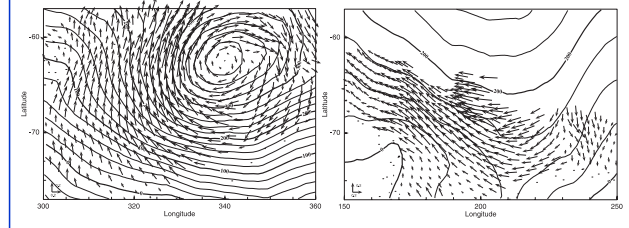
Fig. 2: Streamfunction by FTM in 100 m²/s. Strong zonal components of streamlines correspond sufficiently to drift vectors for both Weddell and Ross sea area.
